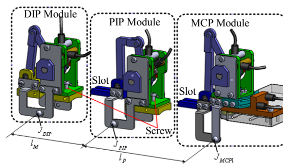
Figure 5. Adjustable connection between joint modules.
