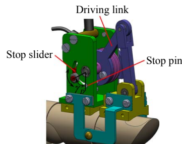
Figure 6. Mechanical stop
