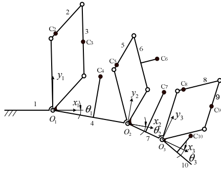
Figure 8. Kinematic sketch of the hand exoskeleton
