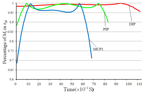
Figure 9. Results of friction experiment.
