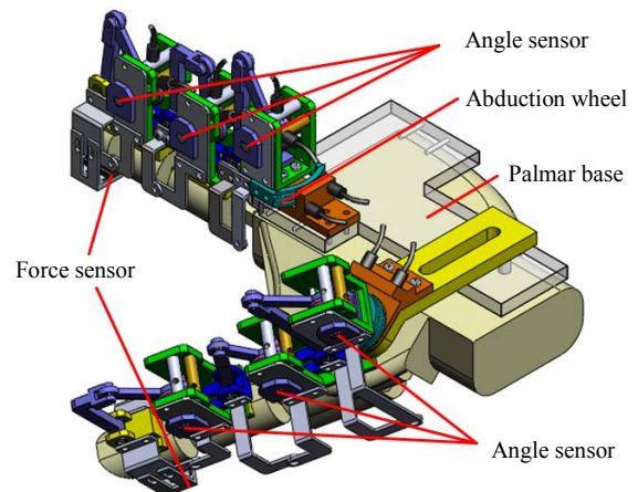
Figure 3. Virtual prototype of the exoskeleton.
